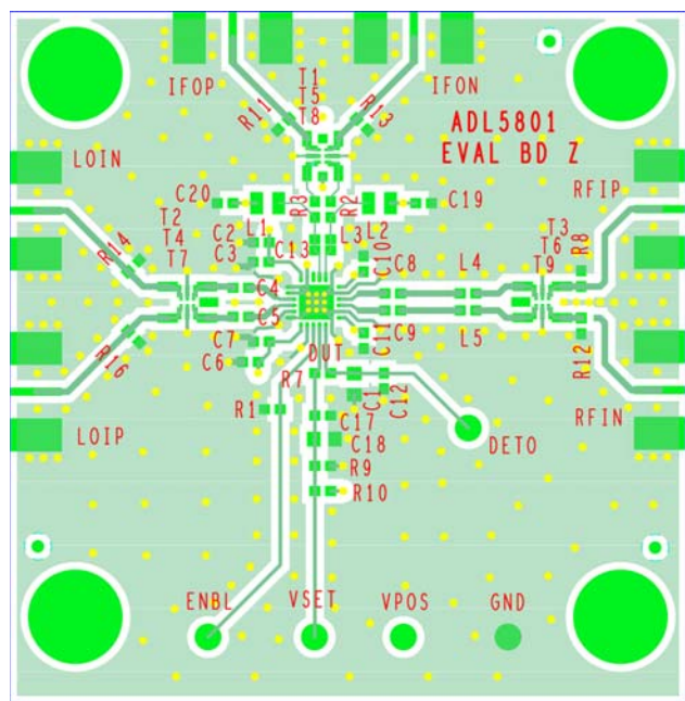
Figure 98. Evaluation Board Top Layer
