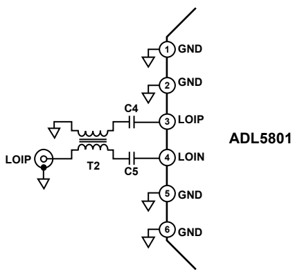
Figure 94. LO Interface
