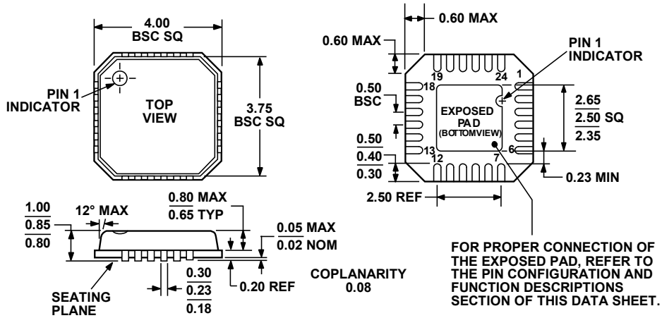
Figure 100. 24-Lead Lead Frame Chip Scale Package [LFCSP_VQ] 4 mm × 4 mm Body, Very Thin Quad (CP-24-3) Dimensions shown in millimeters
