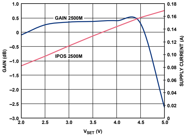
Figure 28. Power Conversion Gain and IPOS vs. V_{SET}
