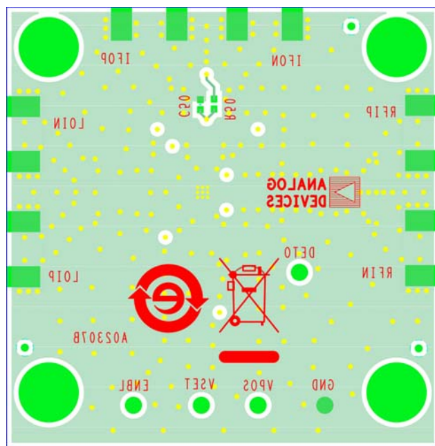
Figure 99. Evaluation Board Bottom Layer
