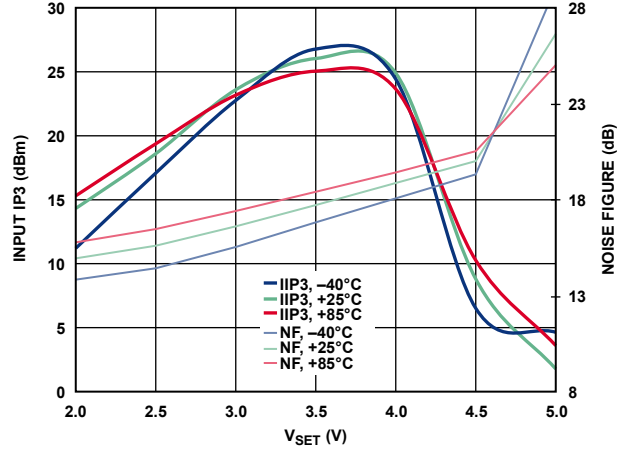
Figure 41. Input IP3 and Noise Figure vs. V_{SET}
