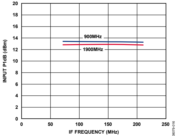
Figure 16. Input P1dB vs. IF Frequency
