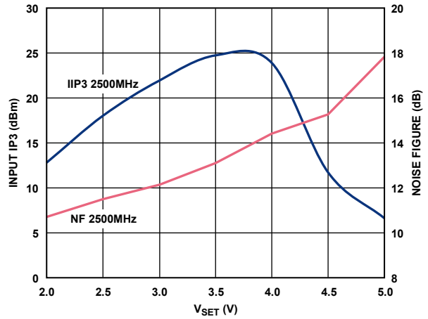
Figure 30. Input IP3 and Noise Figure vs. V_{SET}
