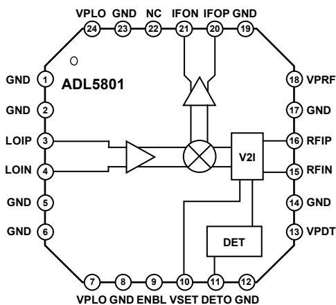
Figure 87. Block Diagram
