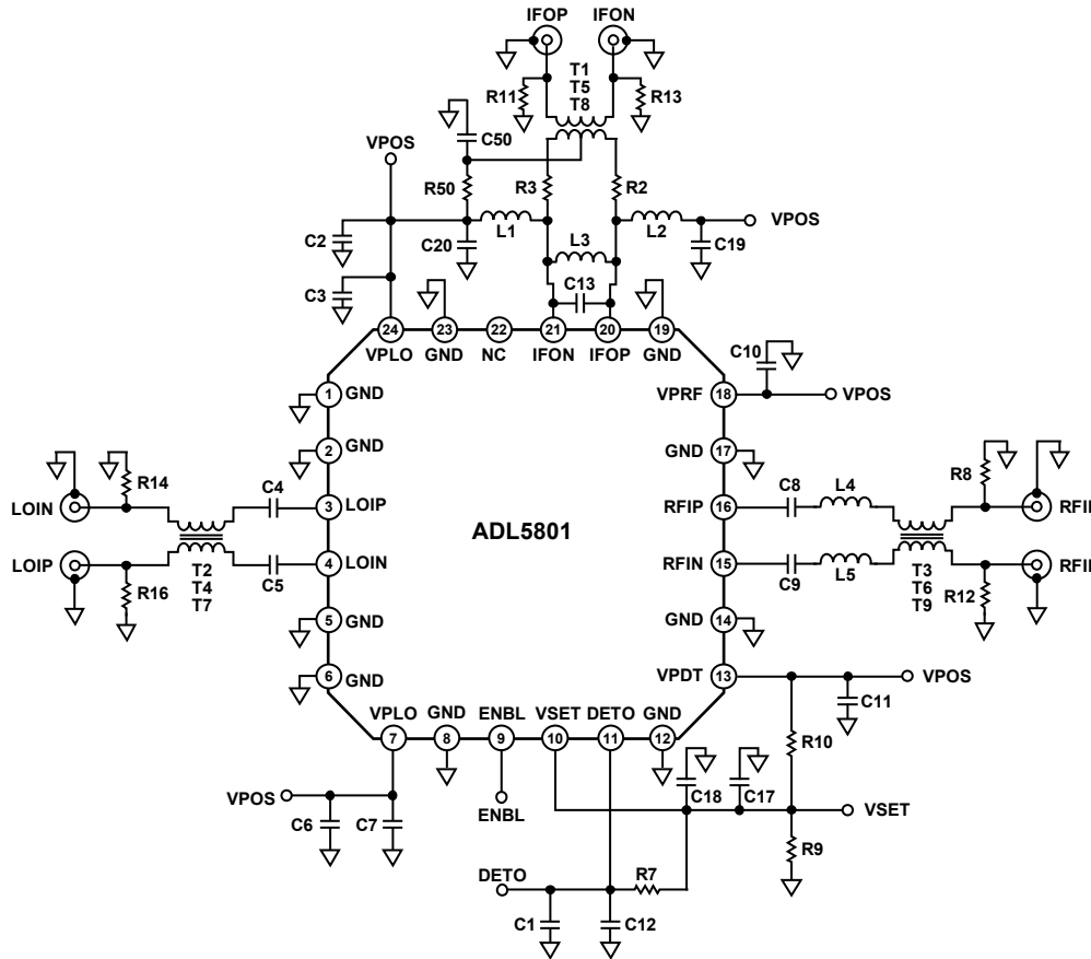
Figure 97. Evaluation Board Schematic
