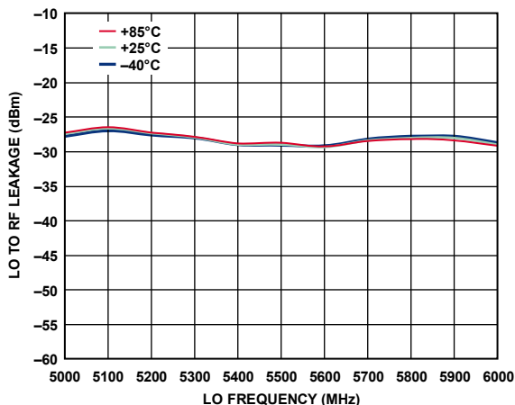
Figure 58. LO to RF Leakage vs. LO Frequency
