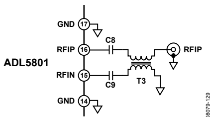
Figure 93. RF Interface
